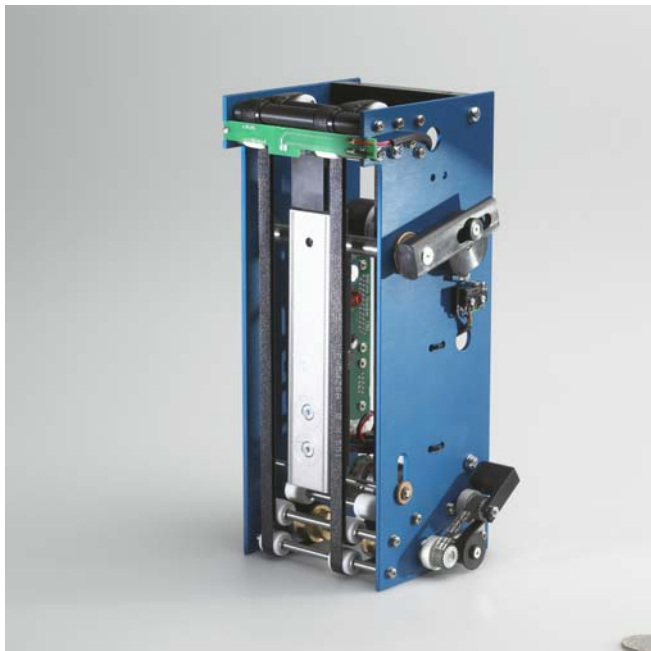
Picture shows BCD-50. This stacker to be used in systems that stacks the note forward. BCD 50 S is to be used when the cash box is in the rear end of the system. BCD 50 stackers are for systems with secure cash box. BCD 50 is a little bit taller than BCD 40.
